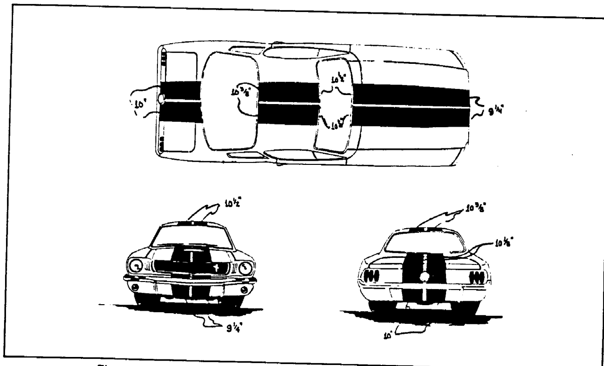
The original Shelby-American LeMans strip dimensions for the '65-66 GT-350. Drawn by Greg Wolf, Shillington, Pa.
